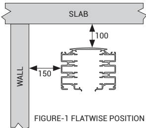
FIGURE-1 FLATWISE POSITION
