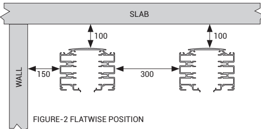
FIGURE-2 FLATWISE POSITION
